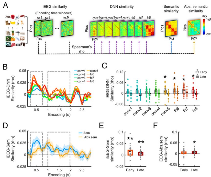
Fig. 3. Distinct representational formats in the early and late encoding clusters. (A) Linking neural representations to visual, semantic, and abstract semantic representations, respectively. Neural similarity matrices were created by correlating activities between all pairs of different pictures in individual encoding time windows. Visual similarity matrices were obtained by correlating activations of the artificial neurons in each DNN layer. The semantic similarity matrix was generated by calculating the cosine similarities of the word vectors between picture labels. An abstract semantic similarity matrix resulted from iteratively regressing out the visual similarity in each DNN layer from the semantic similarity matrix. Exemplar pictures of items from the four categories (animals, fruits, electrical devices, and furniture) used in the study are shown at Left. (B) Correlation (Spearman's rho) between DNN and neural similarity maps for each DNN layer and each encoding time window. Two dashed boxes indicate the time window of the early and the late encoding cluster showing significant item-specific EMS. (C) Averaged correlation between neural similarity in the early and late encoding clusters with the similarity matrices in each DNN layer. Each color dot indicates the correlation value from one participant. (D) Correlation values resulting from comparing the neural similarity with the semantic (blue line) and the abstract semantic similarity (orange line) in each encoding time window. Two dashed boxes mark the time windows corresponding to the early and the late encoding cluster. Color shaded areas around the lines reflect one SEM. (E) Semantic representations correlated with neural representations in both the early and the late encoding clusters. (F) Abstract semantic representations correlated with neural representations in the late encoding cluster. Each color dot indicates one participant. Error bars reflect one SEM. * P < 0.05 ; ** P < 0.01 .
