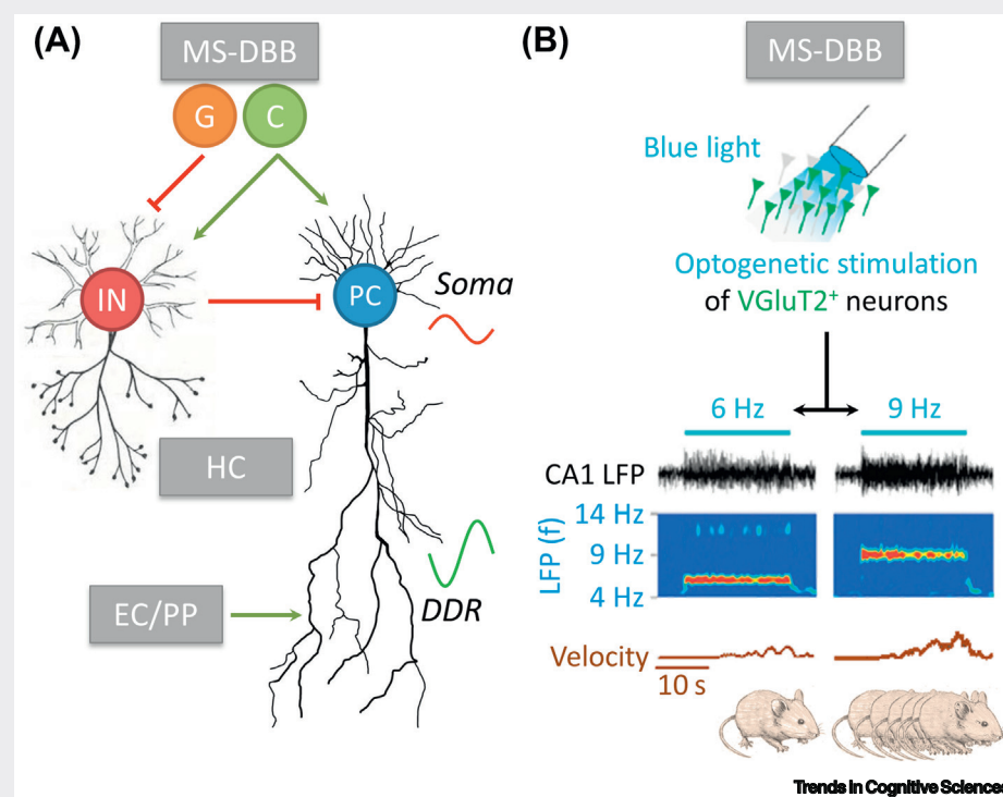
Figure 1. Mechanistic Basis of Theta Oscillations. (A) Classic theta model. See Box 2 text for explanations. Note that many extensions have been suggested to this model. (B) Medial septum and diagonal band of Broca (MS-DBB) VGLUT2 + neurons as a key player in regulating locomotion. Increasing optogenetic stimulation (blue light) frequency of these neurons (from 6 to 9 Hz) leads to higher theta oscillation frequency in CA1 and is followed by increased velocity of the rodent. Abbreviations: C, cholinergic; DDR, distal dendritic region; EC/PP, entorhinal cortex and perforant path; G, glutamatergic; HC, hippocampus; IN, interneuron; PC, pyramidal cell. Adapted from [17] (A) and [34] (B).
