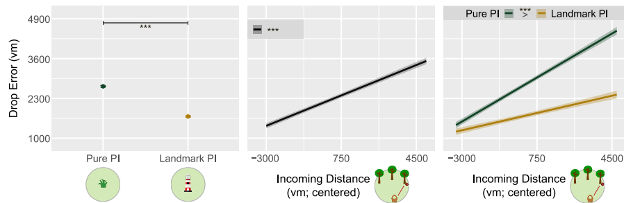
Fig. 4. Effects of stress, subtask, and path distance on general PI performance. (A) Drop error was higher when no spatial cues were available (Pure PI > Landmark PI; left). Higher incoming distances led to higher drop errors (middle) and this effect was stronger in Pure PI than in Landmark PI (right). (B) The effect of stress was more pronounced during Pure PI than Landmark PI (significant interaction), even though post-hoc pairwise comparisons between groups in each condition were not significant (left). The difference in PI performance between both subtasks was larger in the stress group (right). (C) The effect of incoming distance was larger in the stress group. Error bars and confidence bands represent SEM. Pure PI: pure path integration, Landmark PI: landmark-supported path integration, vm: virtual meters, n. s.: not significant, *** p < .001 , ** p < .01 , * p < .05 .
